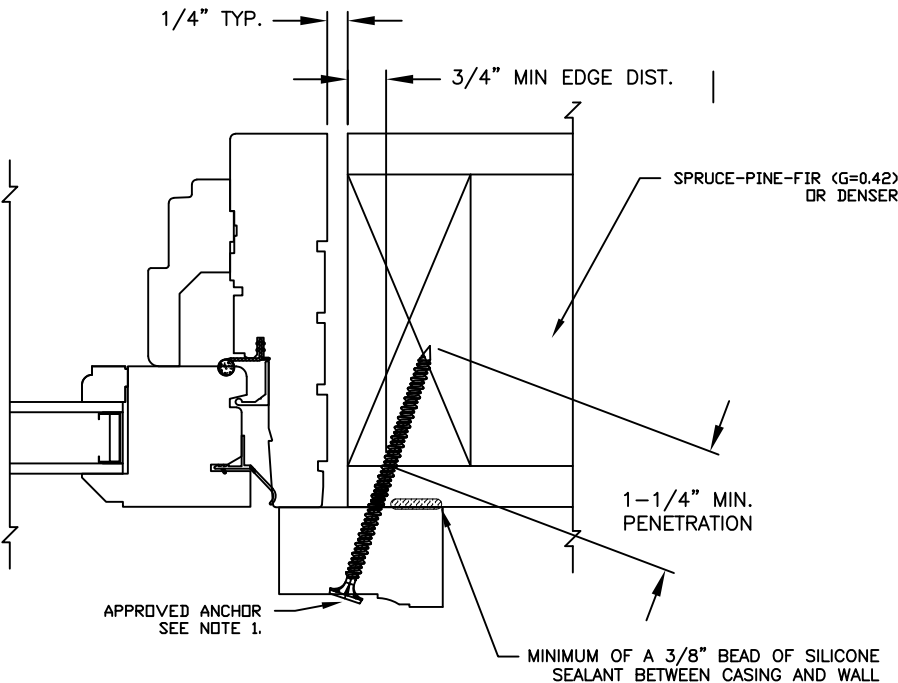
TYPICAL BRICKMOULD/FLAT CASING WINDOW SIDE JAMB
