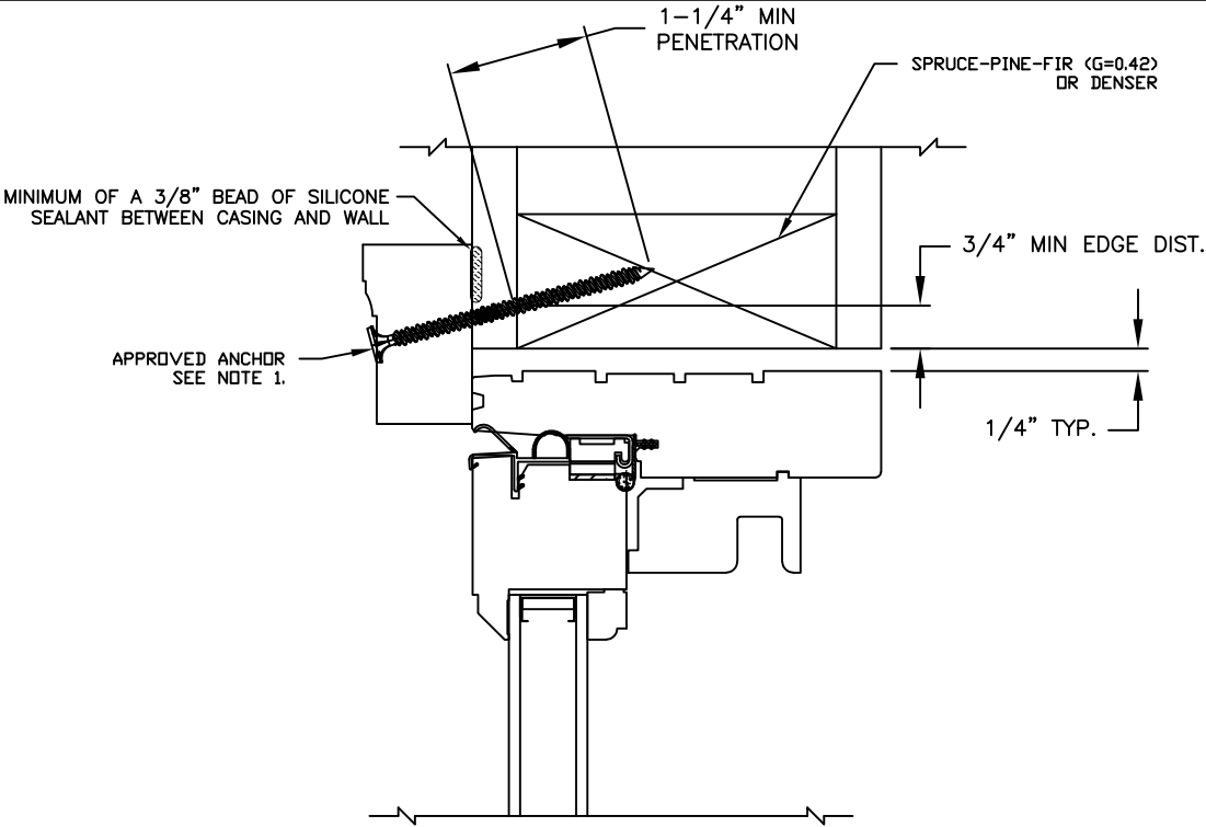
TYPICAL BRICKMOULD/FLAT CASING WINDOW HEAD JAMB
